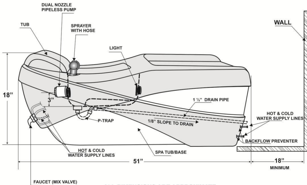
ALL DIMENSIONS ARE APPROXIMATE SIDE VIEW
