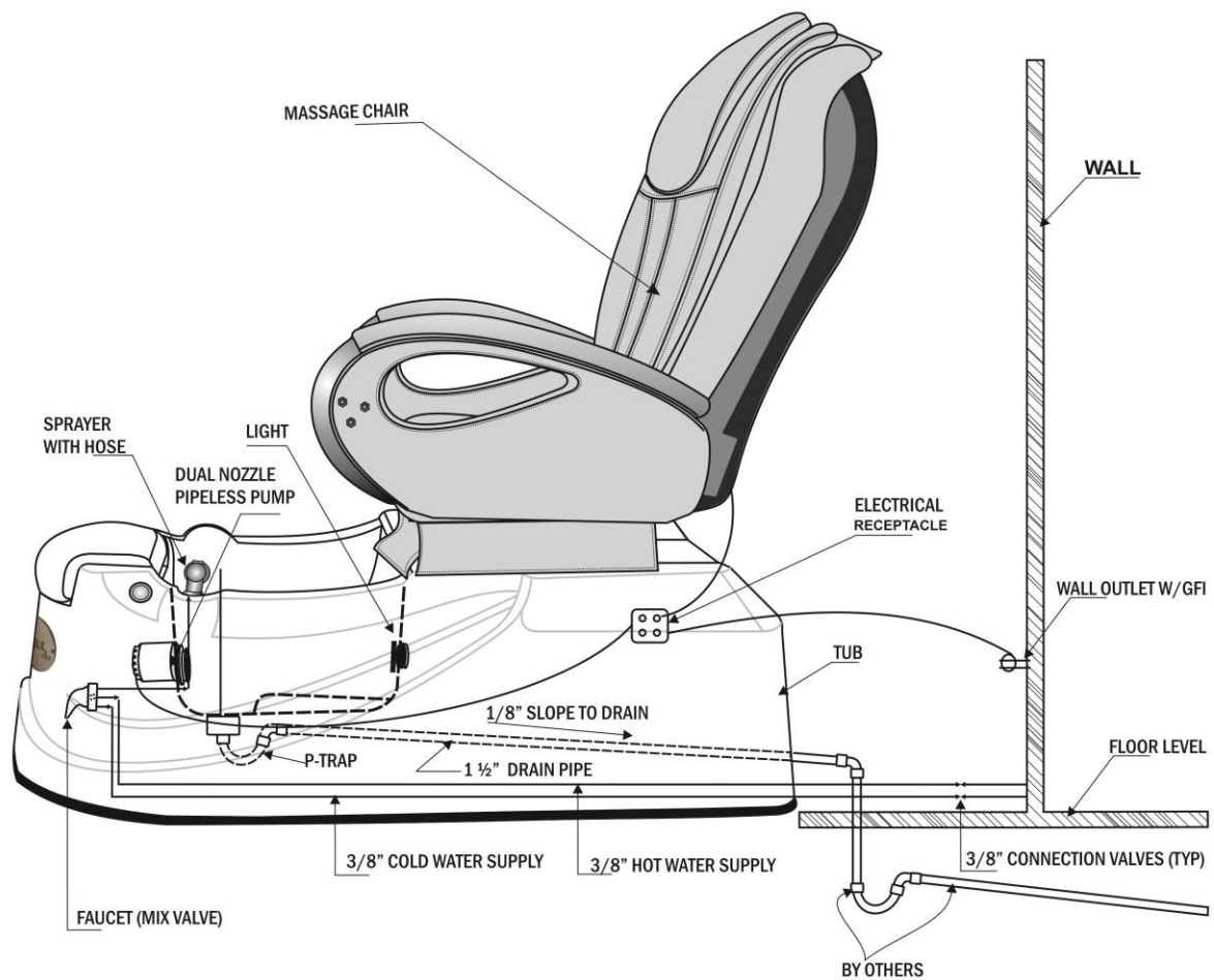
GRAVITY DRAIN INSTALLATION
